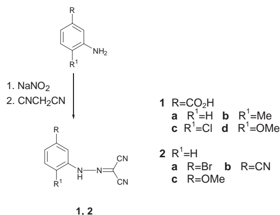
Scheme 1 Synthesis of compounds 1 and 2 .
